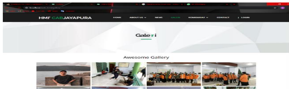
Gambar 4.4 Form Galeri
