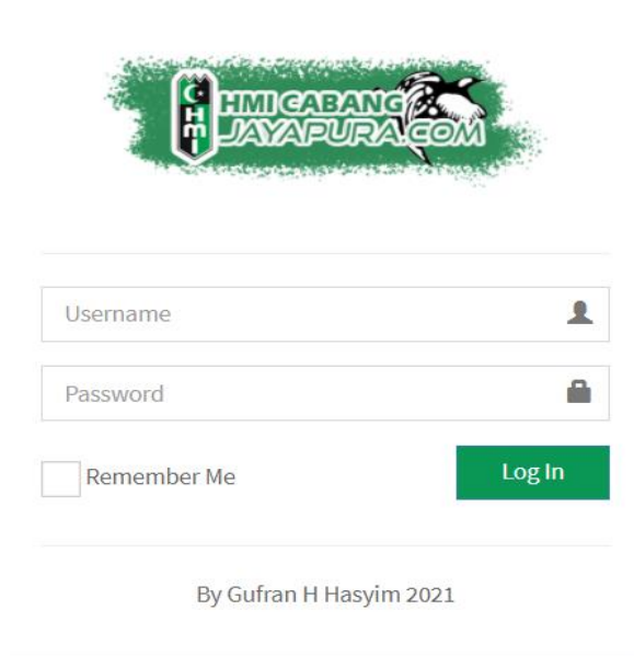
Gambar 4.6 Form Login
