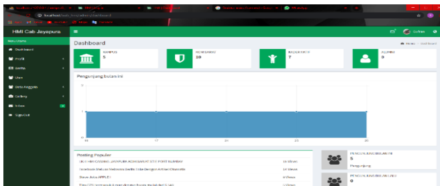
Gambar 4.7 Menu Dasboard
