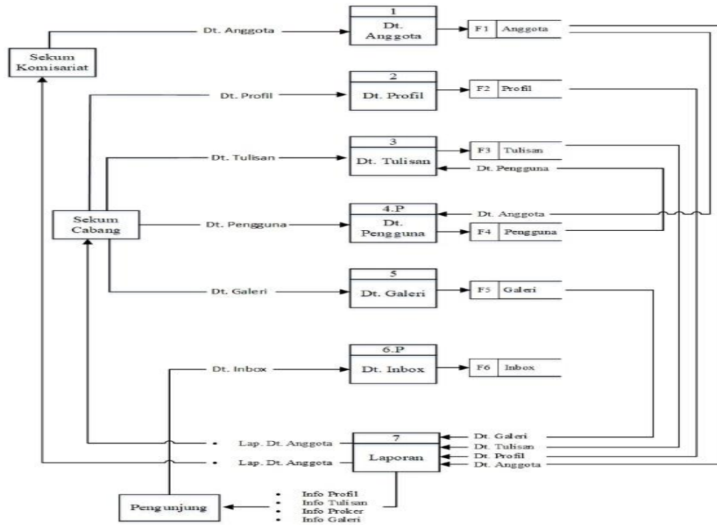
Gambar 3.3 Diagram Overview level 0
